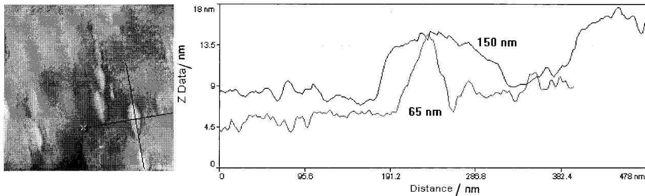
Figure 4. Cross-sections of an aggregate at the surface of a sample with 7.2 wt % of R812.
