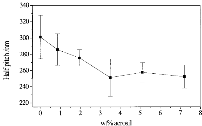
Figure 7. Half pitch from line measurements of the AFM images.
