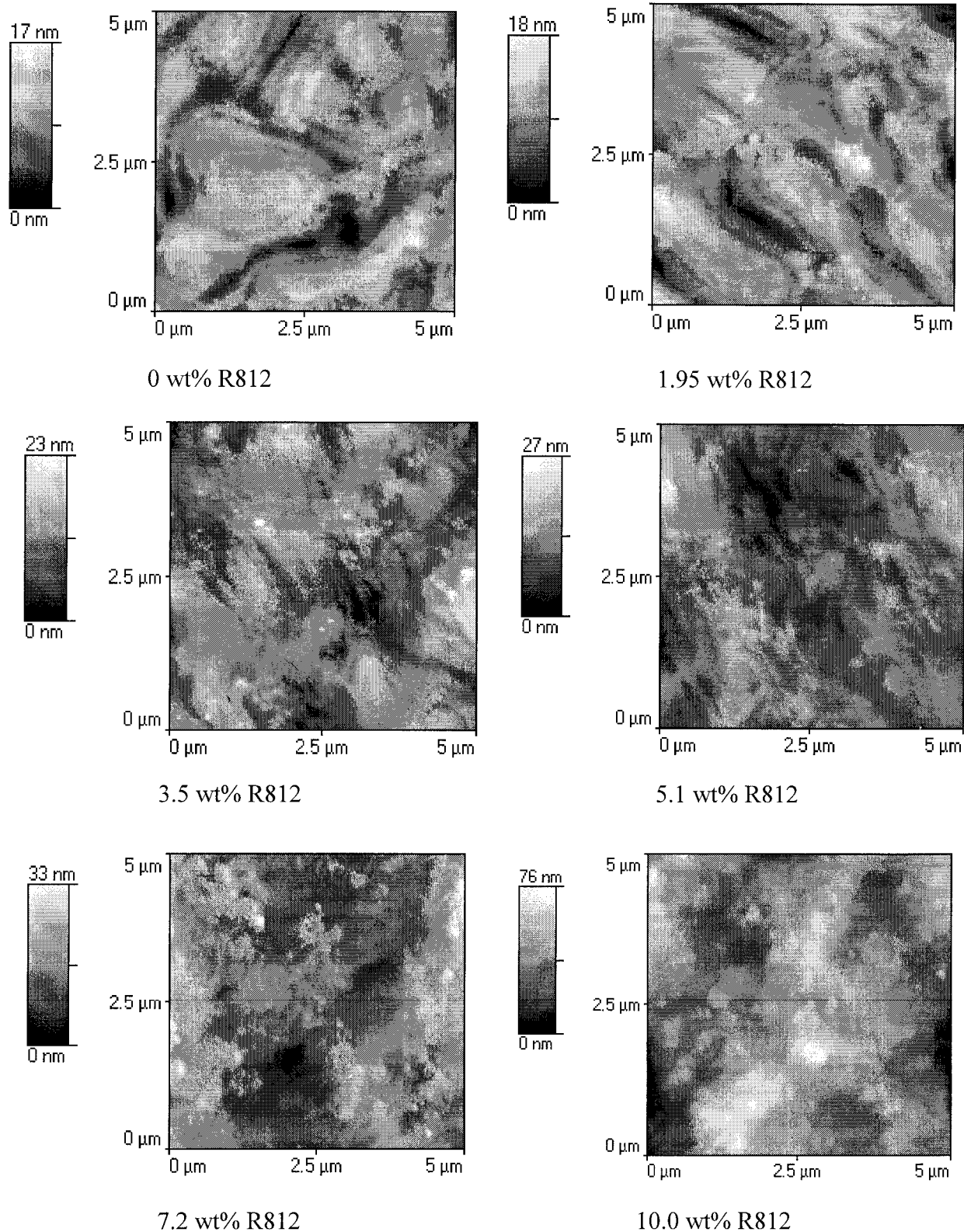
Figure 1. AFM images of the cholesteric liquid crystalline matrix C4762L at different aerosil R812 concentrations.
