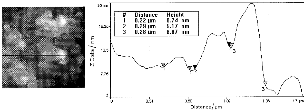
Figure 3. AFM image and line measurement (cross section) of the sample with 10 wt % R812. Inset data relate to the distance and height differences between points on the line indicated by the differently numbered pairs of inverted triangles.
