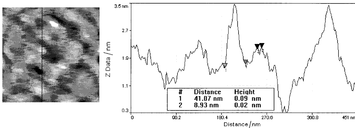
Figure 5. Line profile in the AFM image of the sample with 3.5 wt % R812. Inset data as described in the legend to figure 3.
