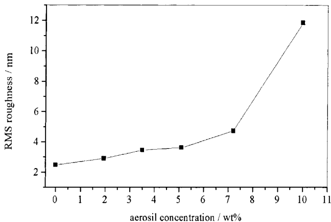
Figure 2. RMS roughness values of the AFM images from figure 1 versus aerosil concentration.
