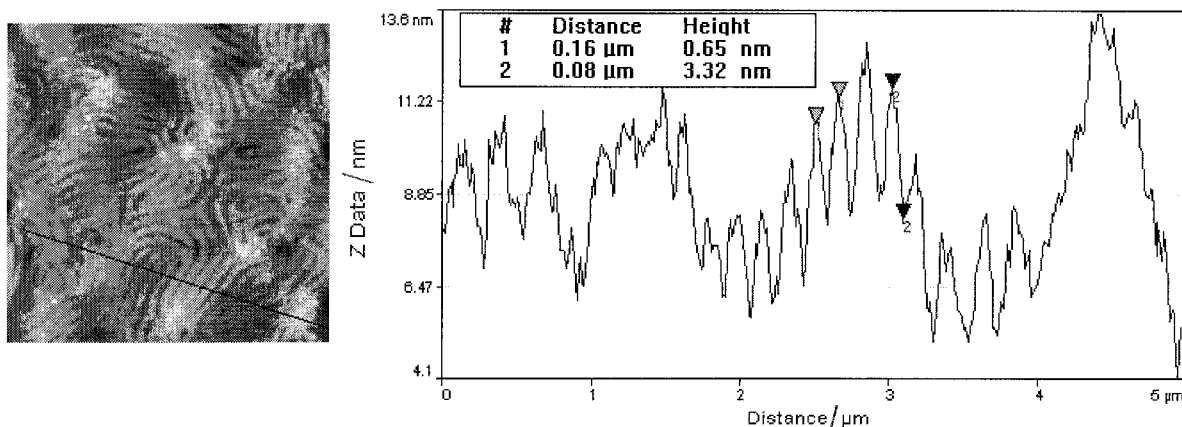
Figure 6. Line measurement of the AFM image of the sample with 5.1 wt % R812. Inset data as described in the legend to figure 3.
